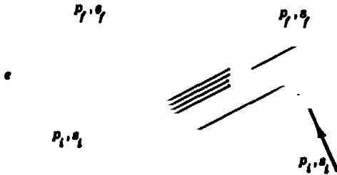
Fig. 7-8 Coulomb scattering of electrons.
