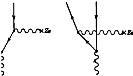
Fig. 7-18 Pair production in a Coulomb field.
