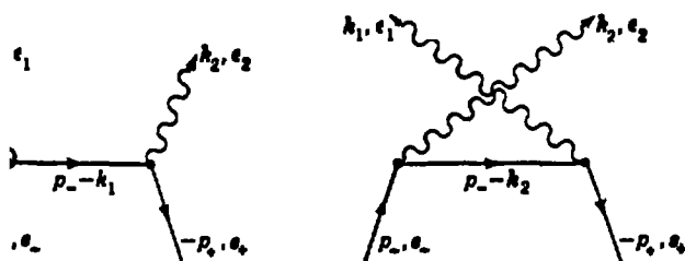
Fig. 7-11 Pair annihilation.
