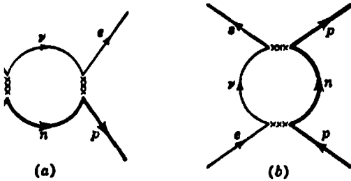
Fig. 10-16 Some higher order graphs for \beta decay.
