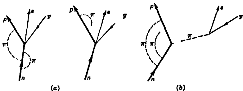
Fig. 10-23 Weak axial contributions to \beta decay.
