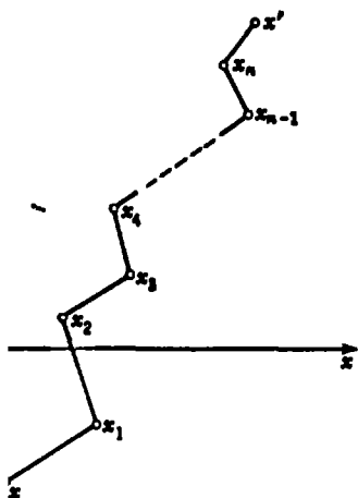
Fig. 6-4 n th order contribution to G(x, x') .
