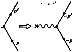
Fig. 10-24 Weak-interaction vertex of an antiproton.
