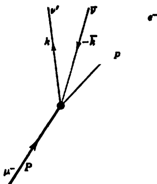
Fig. 10-17 \mu decay.
